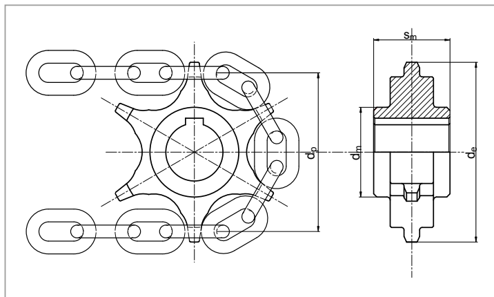
Ruota dentata - Toothed wheel - Rueda dentada
